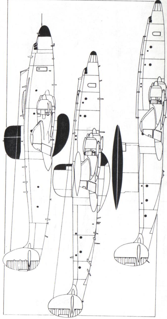
Top to bottom Lockheed WV-2/EC-121K, WV-2E/EC-121L
